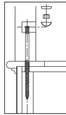
3008-10 NEWEL POST FASTENER 10-3/4" anchor bolt
