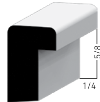
280 BACK BAND 11/16 x 1-1/16 PRIMED RL PINE 8' Fits up to 11/16 Profile
